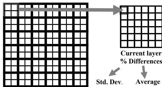
Appendix Figure 3: From the differences among the 2 element x 2 element previous layer create a data base to be used as the basis for the current layer mottle measurements. The standard deviation and average of these are two terms in the mottle calculation.
